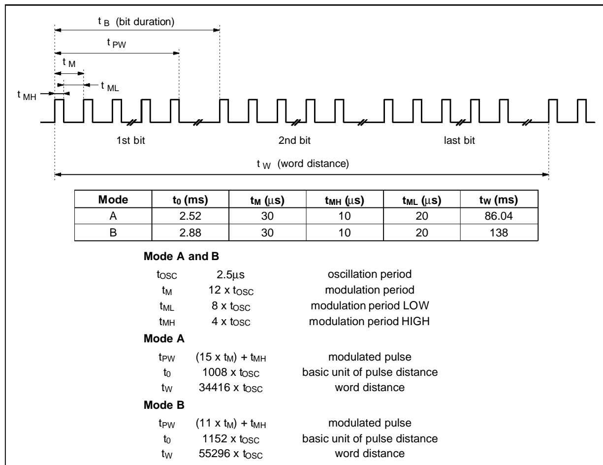
Figure 2 : Pulse Train Timing (ref. to f osc = 400kHz)
