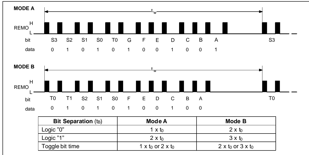
Figure 2 : Pulse Train Timing (ref. to f osc = 400kHz)
